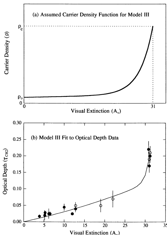
FIG. 5.—(a) Density distribution of the carbonaceous carrier assumed in Model III, i.e., the local density of -\text{CH}_2- absorber is \rho_0 and the density increases exponentially as one approaches the Galactic center. (b) Comparison between the optical depth function of the 2925\text{ cm}^{-1} band and Model III using the parameter values given in Table 2 (see text for details). The points have the same meanings as given in Fig. 1.
