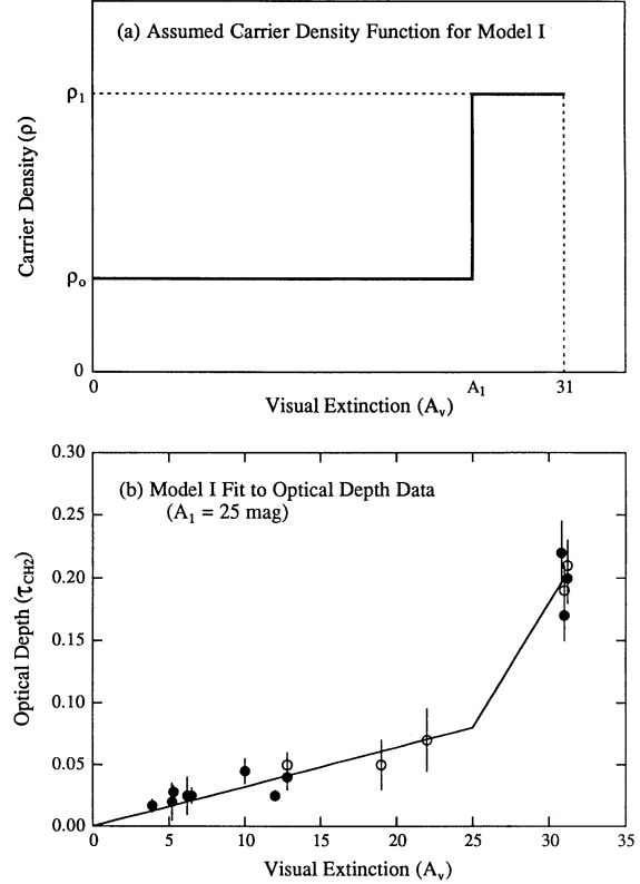
FIG. 3.—(a) Density distribution of the carbonaceous carrier assumed in Model I, i.e., the density ( \rho_0 ) of -\text{CH}_2- absorber is constant everywhere except in a limited region around the Galactic center, where the material is present at a higher density ( \rho_{\text{GC}} ). (b) Comparison between the optical depth function of the 2925 \text{ cm}^{-1} band and Model I using the parameter values given in Table 2, A_1 = 25 \text{ mag} , and \rho_{\text{GC}} = 0.02 \text{ }-\text{CH}_2-\text{ cm}^{-2} \text{ mag}^{-1} (see text for details). The points have the same meanings as given in Fig. 1.
